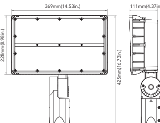
135W&200W(Slipfitter Mount)
