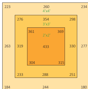
GL02640W 2.7µmol/J 36"/900mm Height
