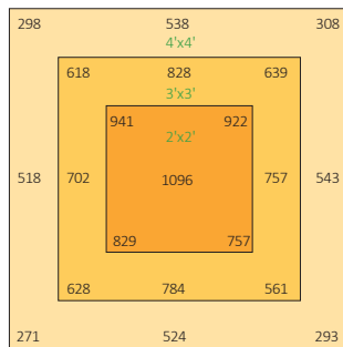
GL02640W 2.7µmol/J 12"/300mm Height
