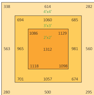
GL02640W 2.7µmol/J 6"/150mm Height
