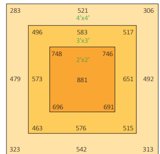
GL02640W 2.7µmol/J 18"/450mm Height
