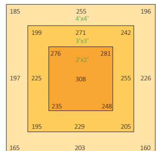
GL02640W 2.7µmol/J 48"/1200mm Height
