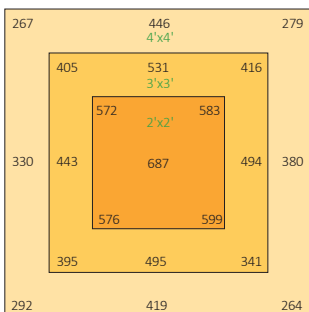
GL02640W 2.7µmol/J 24"/600mm Height
